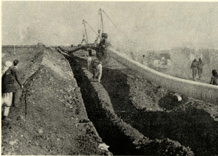
Constructing the I. P. C. pipeline in Northern Lebanon. The coat and wrap machine in operation.
